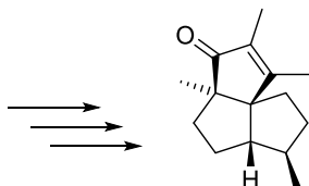
(-)-silphiperfol-6-en-5-one
